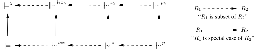
Figure 1: Relationships between probabilistic and ordinary formalisms.
