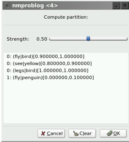
Figure 6: Window for computing the z_\lambda -partition.
