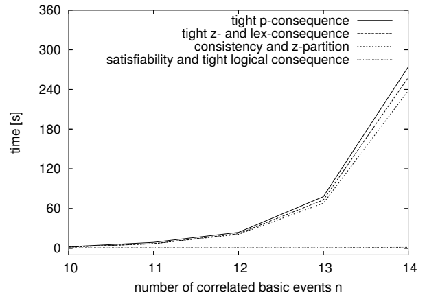
Figure 8: Time used by NMPROBLOG for different reasoning tasks on a chain of n correlated basic events ( 2^n worlds).
