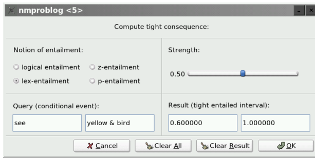
Figure 7: Window for computing tight entailed intervals.
