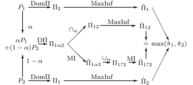
Figure 2: Objective possibilities. D\Pi = \text{Dom}\Pi = dominating possibility measures. MI = \text{MaxInf} = maximally informative possibility measure. \cap_\alpha = intersection over all \alpha in [0,1] . \cup_\alpha = union over all \alpha in [0,1] . Other symbols as in text.
