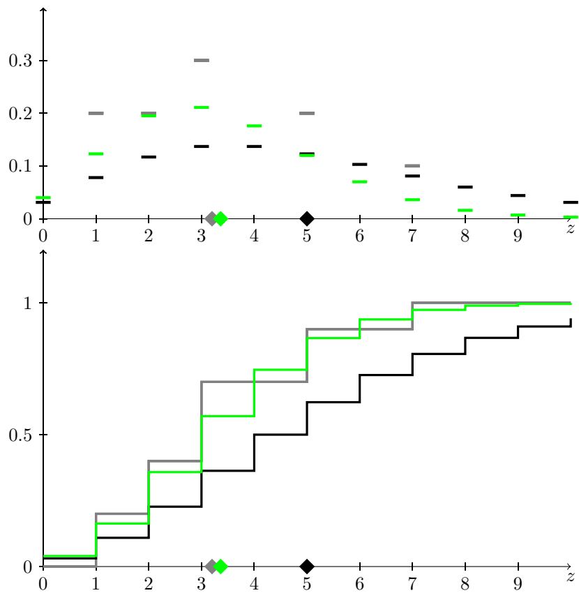
FIGURE 12. Probability mass function plot and cumulative distribution function plot for the Gamma-Poisson model with s := 1 : prior (in black) and the corresponding posterior (in green).
