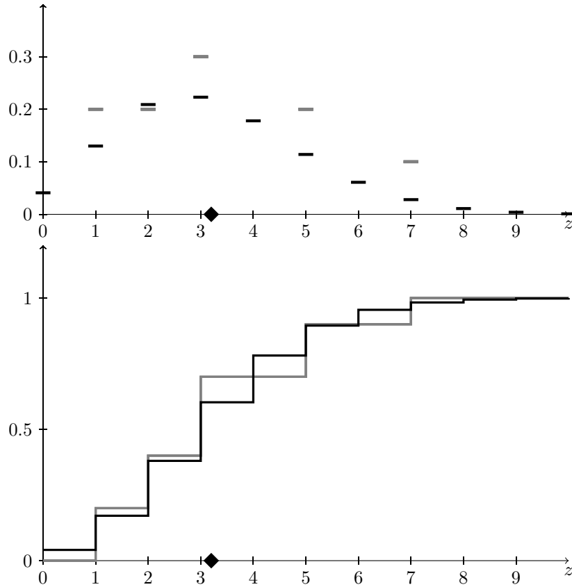
FIGURE 6. Probability mass function plot and cumulative plot for the Poisson model with sample mean value as the parameter value.
