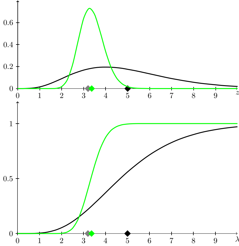
FIGURE 8. Probability density function plot and cumulative distribution function plot for the Gamma model with s := 1 : prior (in black) and the corresponding posterior (in green).
